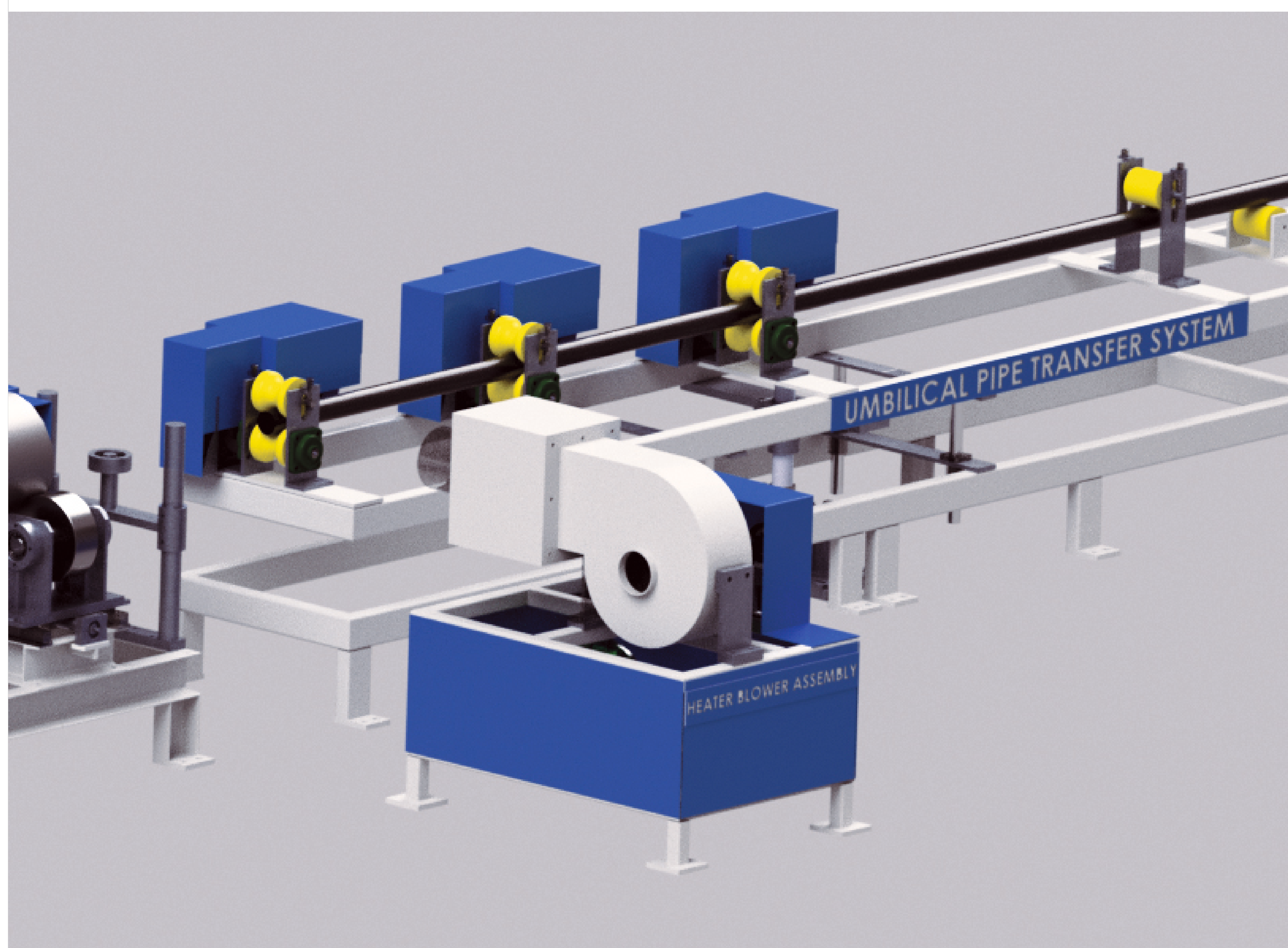
Umbilical Hose Pipe 10m Long
